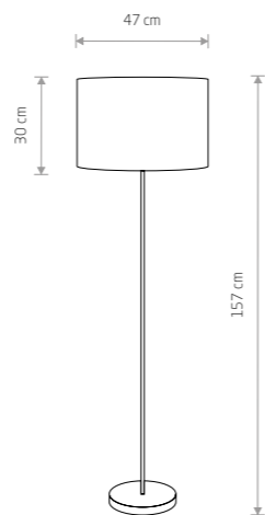
HOTEL fabric, chrome plated steel
