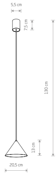
ZENITH S painted steel, solid brass
