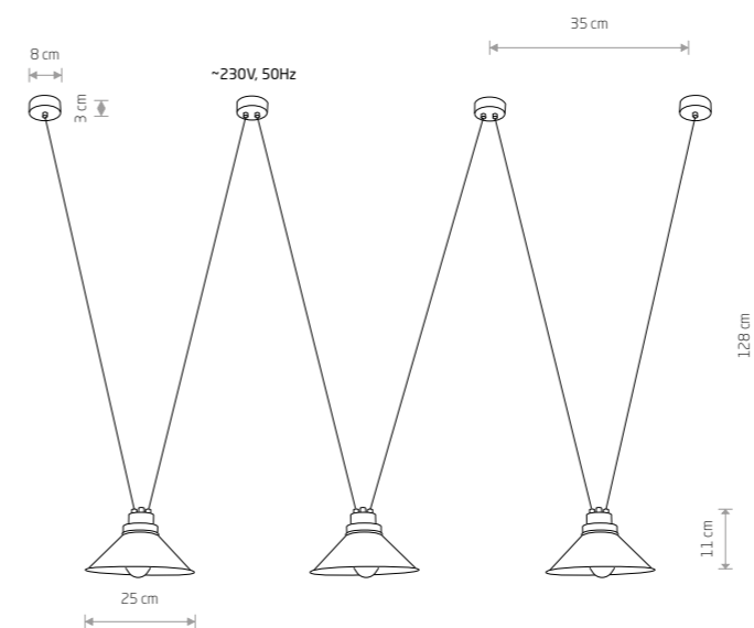
PERM painted steel
