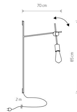
AXIS painted steel
