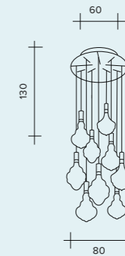
LED 47,7W - 500 mA 3000°K / 3816 lumen
